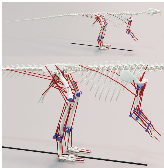
FIGURE 2 The completed musculoskeletal model including the muscle-tendon units (red), joints (yellow), wrap cylinders for guiding the muscles over the bones (blue), and contact spheres for interacting with the floor (green). This bipedal stance was used as the starting point for the initial simulations. The final rendering was produced using NVIDIA Omniverse. Scale bar = 0.5 m, total body length \approx 1.35 m.
