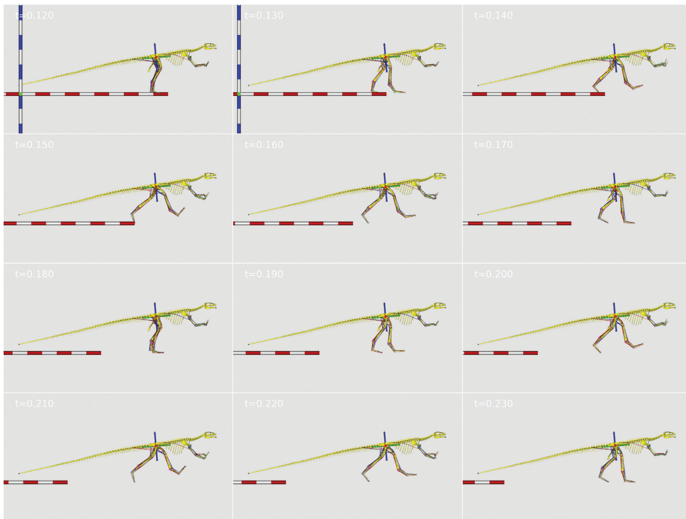
FIGURE 5 Snapshots from the bipedal simulation of Scutelosaurus where gait was optimized for the maximum distance traveled in 3 s with no constraint on metabolic energy available. t indicates time in seconds.
